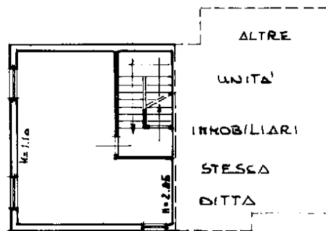
PIANO SOFFITTA
