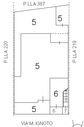
PIANO TERRA
