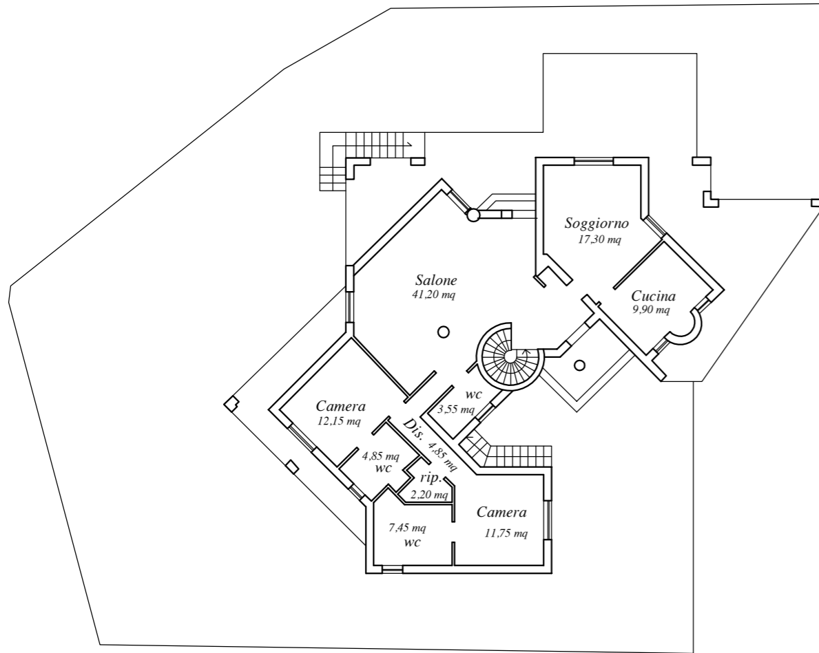
Piano Terra
