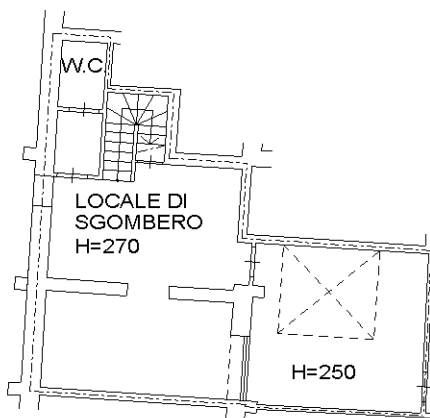
PIANO INTERRATO
