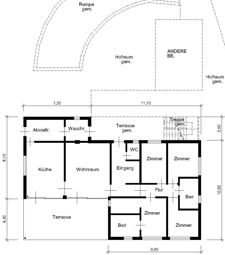
ERDGESCHOSS - PIANO TERRA H = 2.60m
