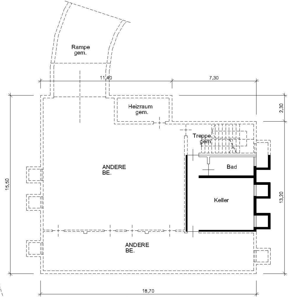
KELLERGESCHOSS - PIANO INTERRATO H = 3.00m
