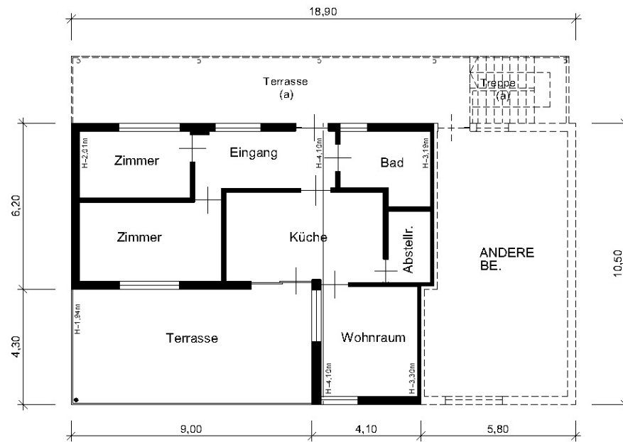
OBERGESCHOSS - PRIMO PIANO H = 1.94-4.10m
