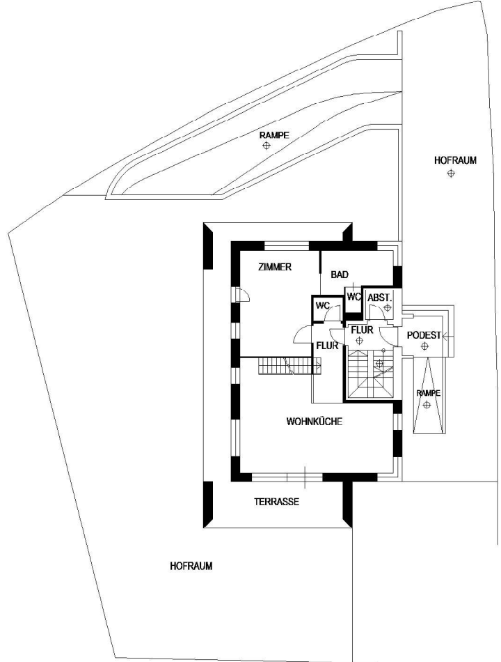
ERDGESCHOSS H=2,40m
