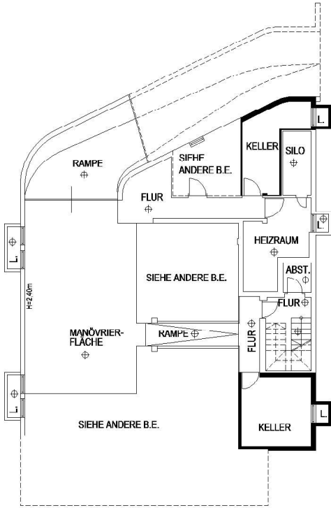
KELLERGESCHOSS H=2,40m
