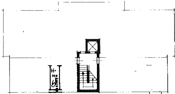
PIANO INTERRATO
