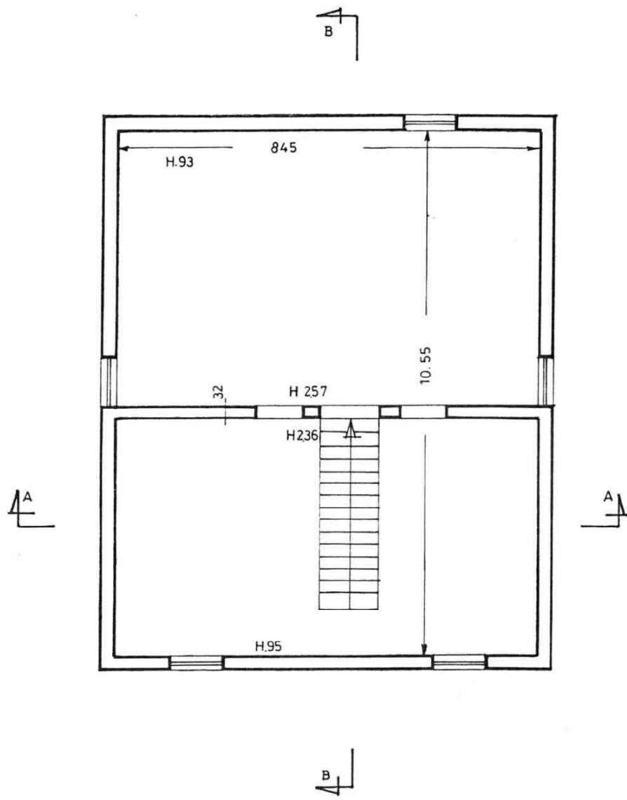
PIANO SOFFITTA
