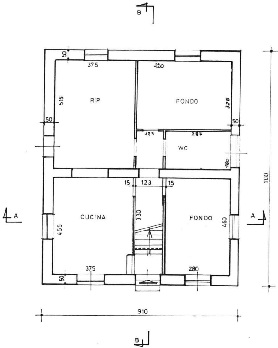
PIANO TERRA
