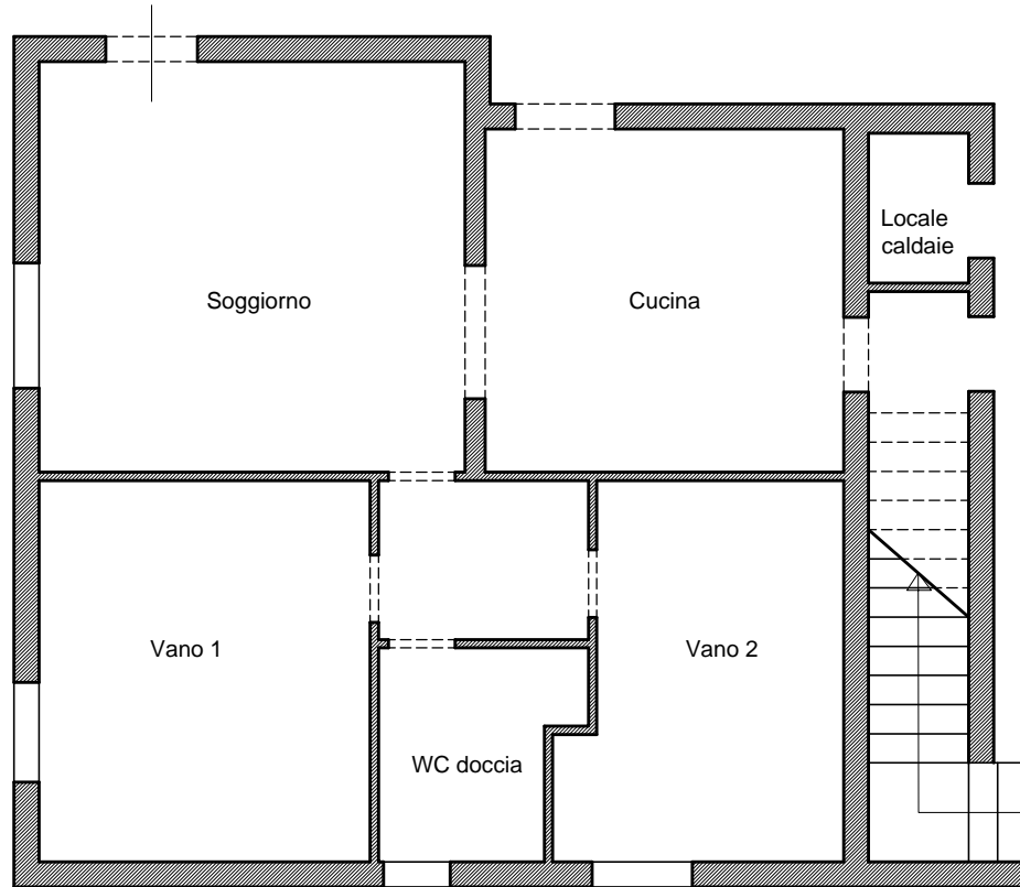
Piano terra - scala 1/100
