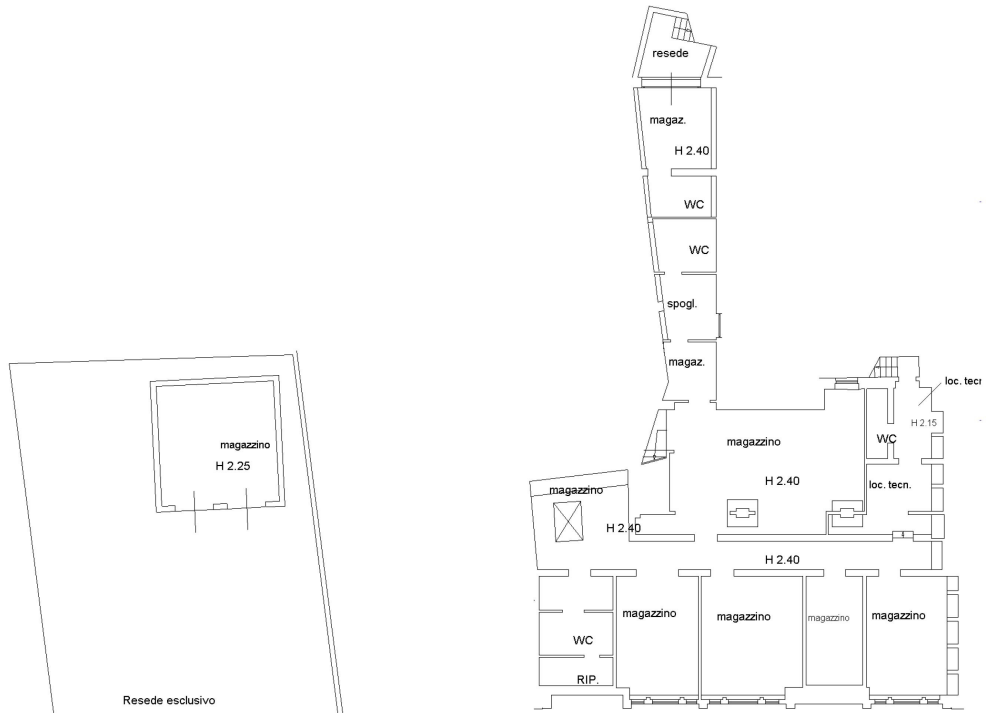
PIANO SEMINTERRATO
