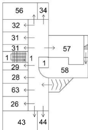
PIANO INTERRATO
