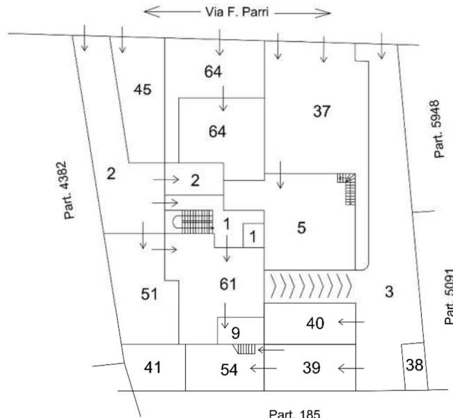
PIANO TERRA
