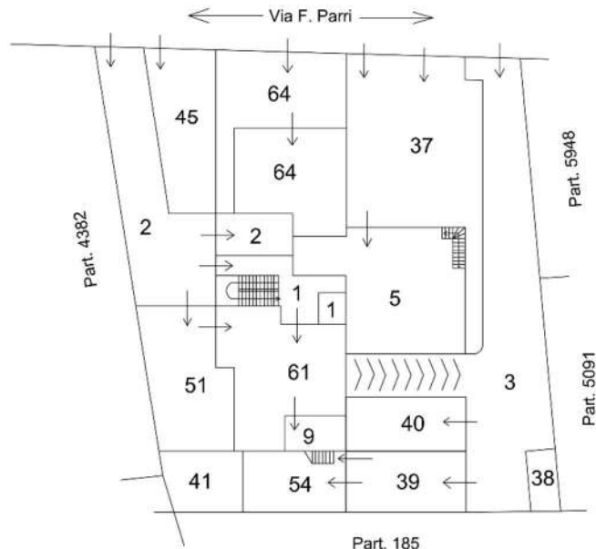
PIANO TERRA
