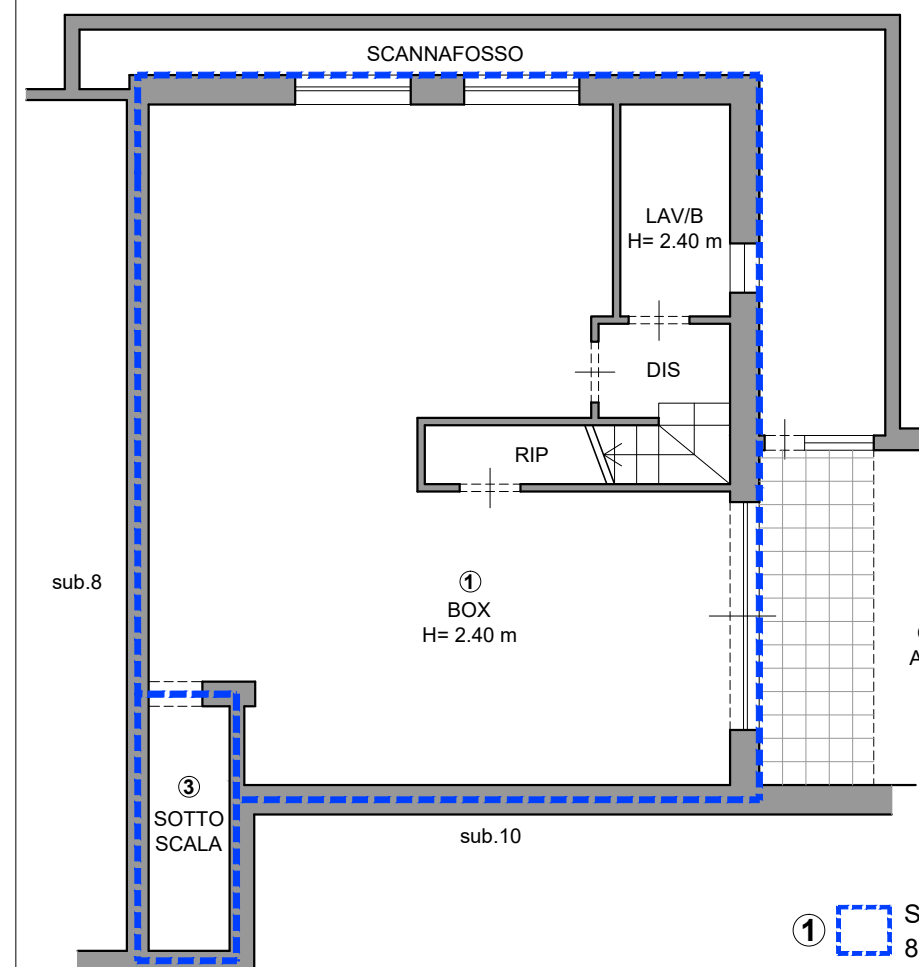
PLANIMETRIA PIANO SEMINTERRATO
