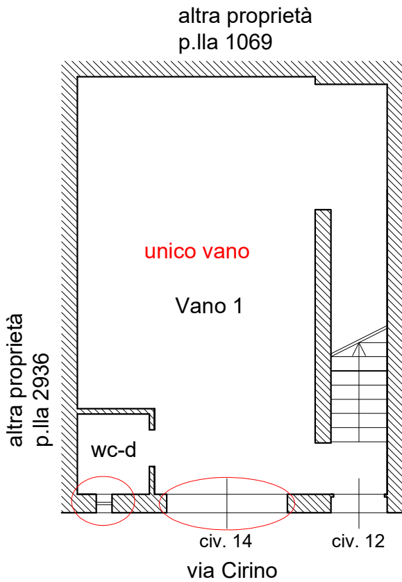
PIANO TERRA
