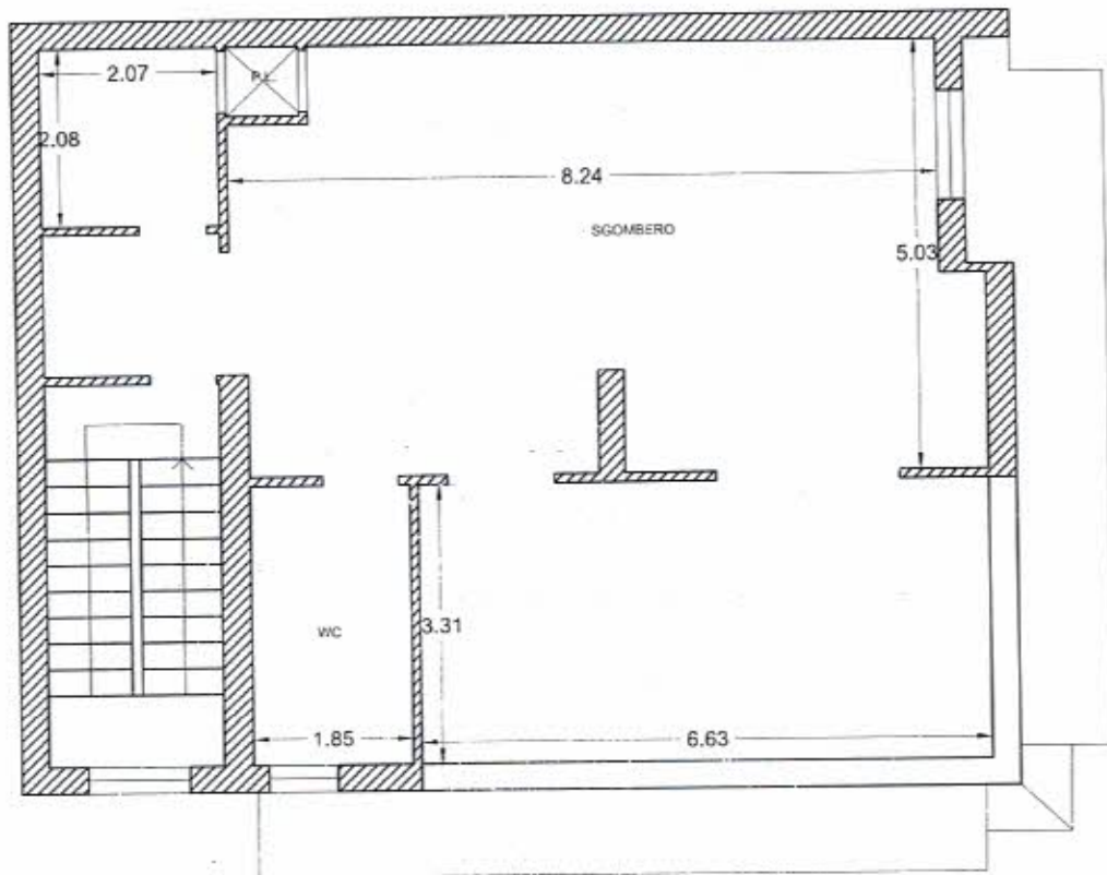
piano piano terzo _ scala 1:100
