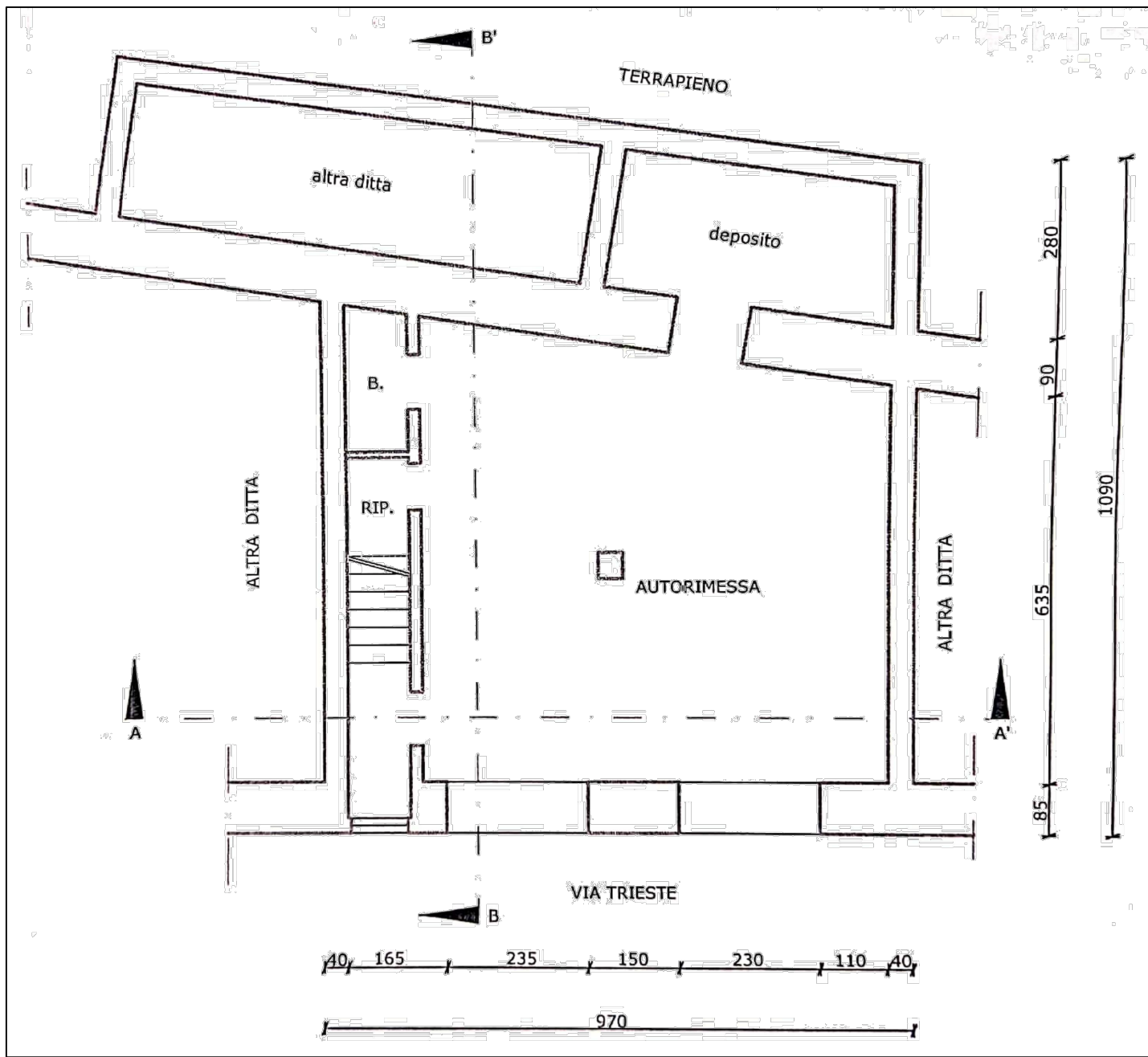
PIANO TERRA H=3,50m.
