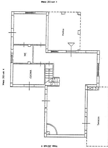
PIANO TERRA H= 2.72ml
