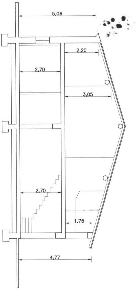
PIANO TERRA
