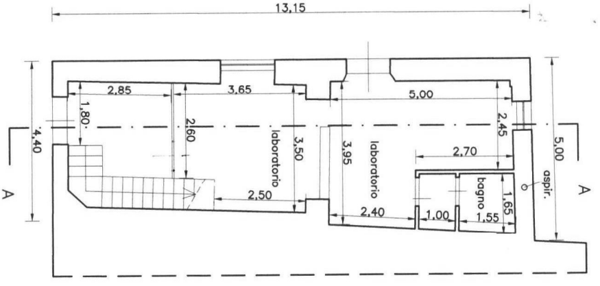
PIANO TERRA
