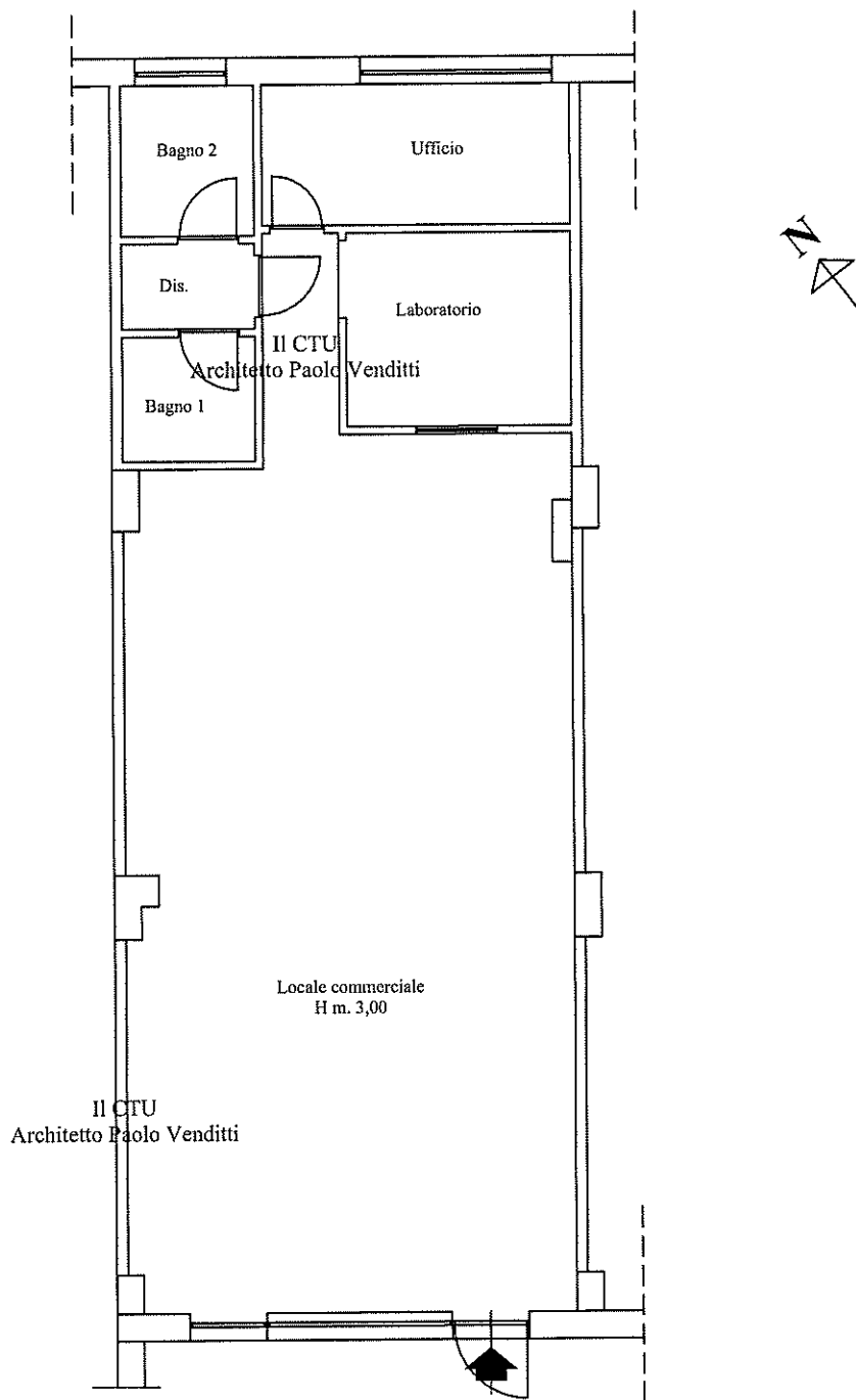
PLANIMETRIA PIANO TERRA
