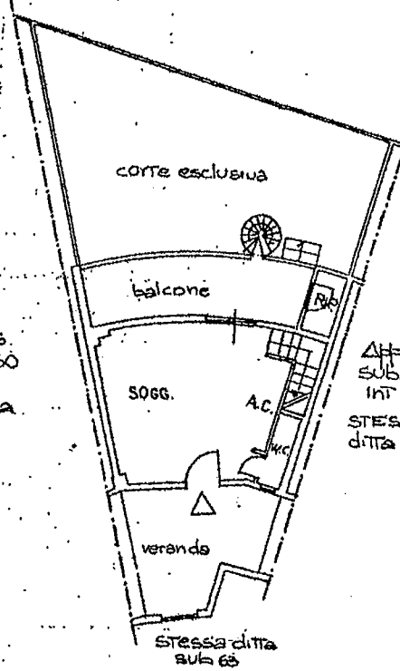
PIANTA PIANO TERRA H=ML. 2.70
