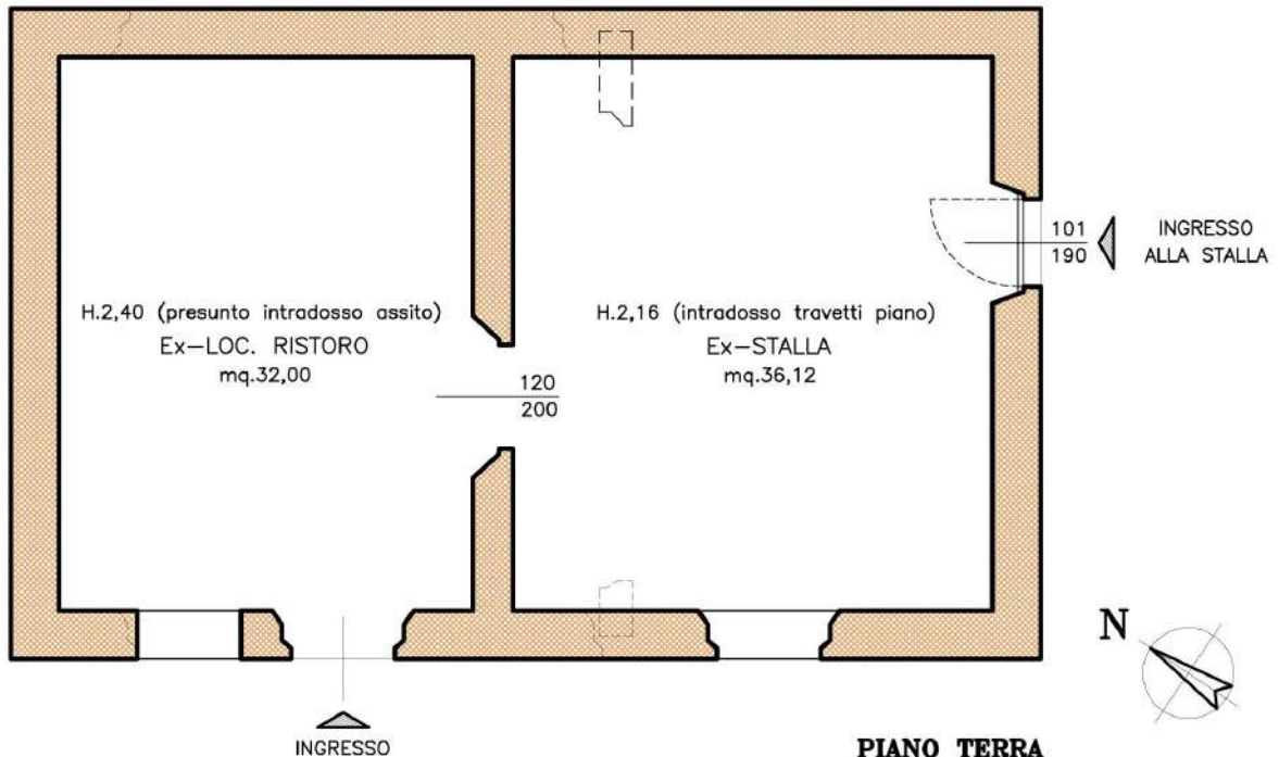
PIANO TERRA
