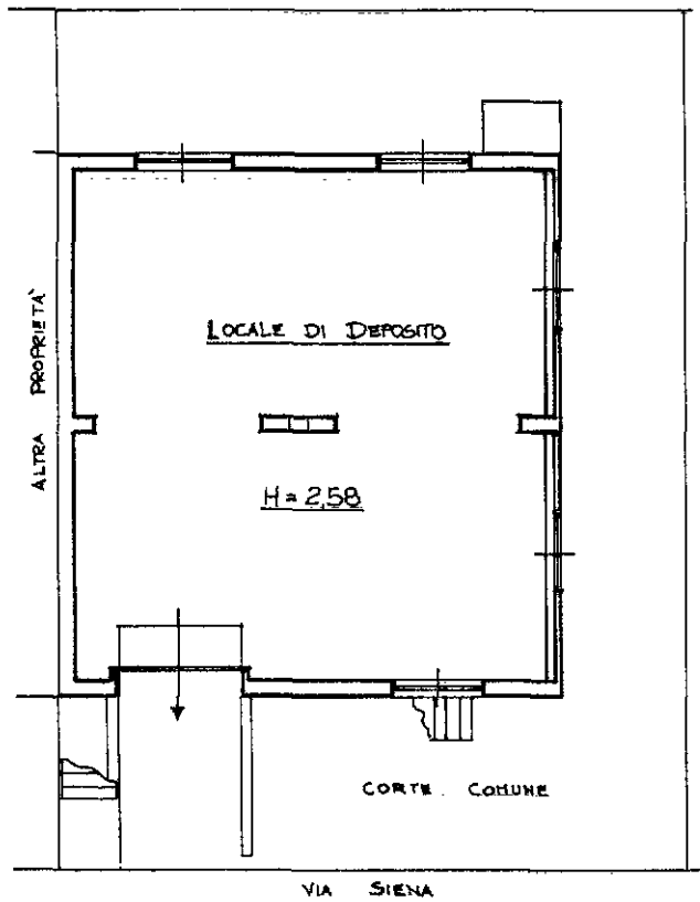
PIANO SEMINTERRATO
